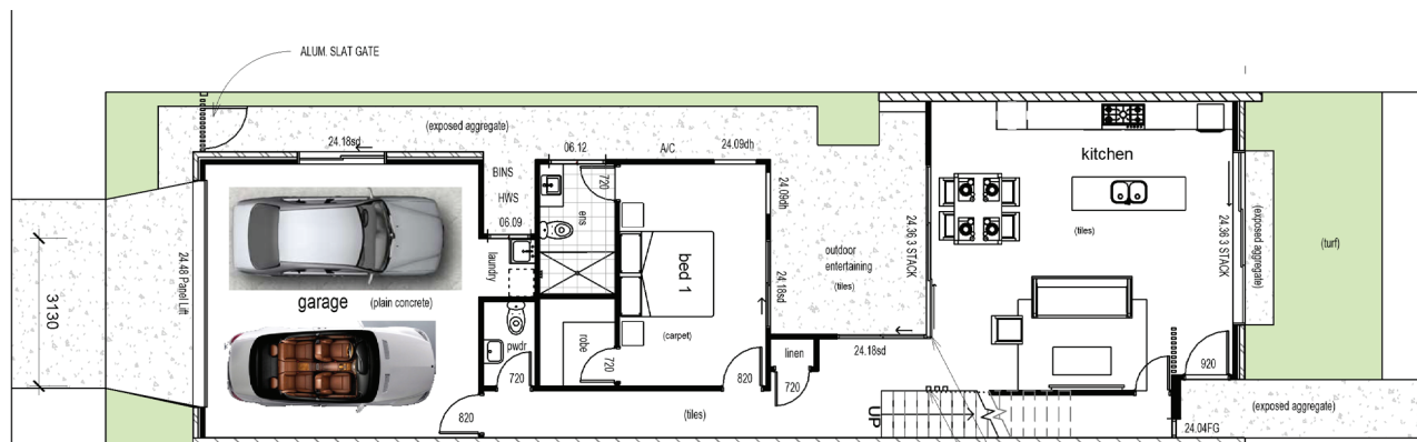
LOWER FLOOR PLAN
