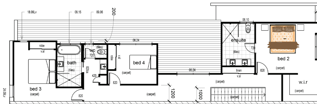
UPPER FLOOR PLAN
