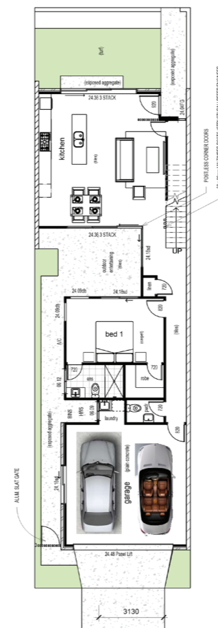
LOWER FLOOR PLAN
