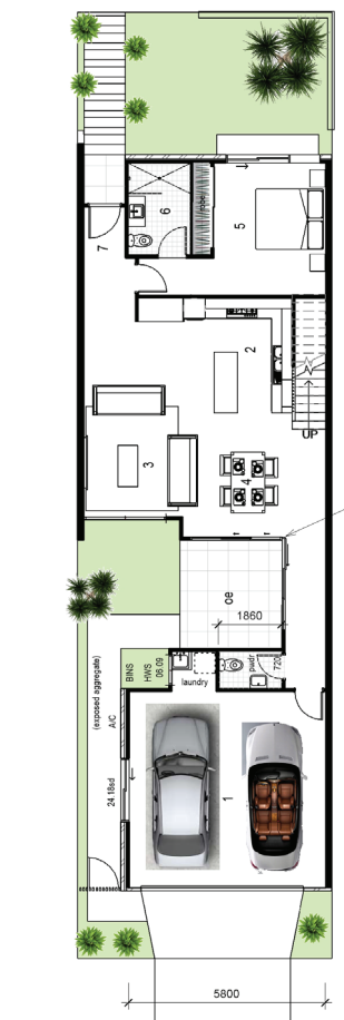
LOWER FLOOR PLAN
