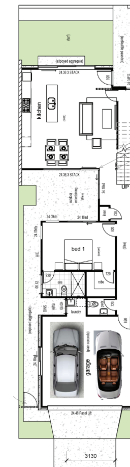
LOWER FLOOR PLAN
