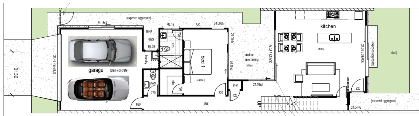
LOWER FLOOR PLAN
