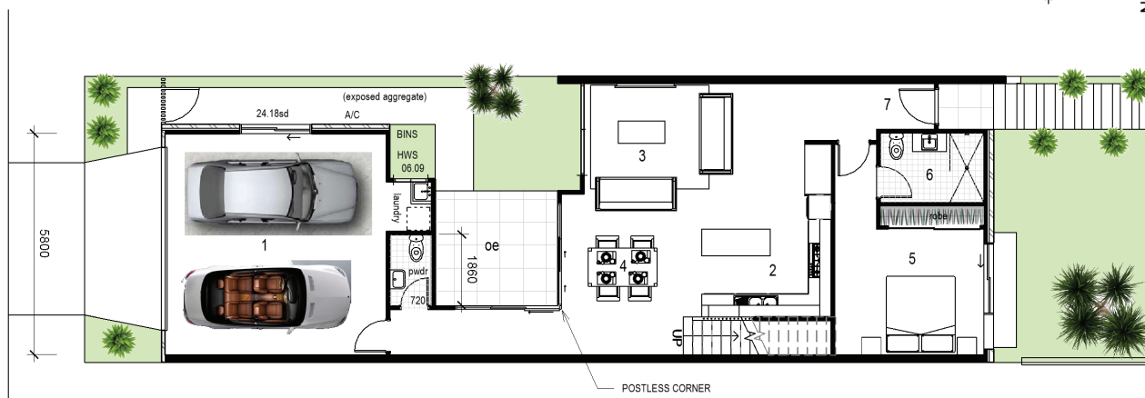
LOWER FLOOR PLAN
