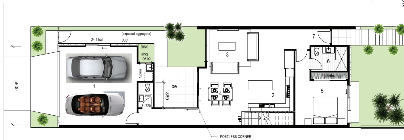
LOWER FLOOR PLAN
