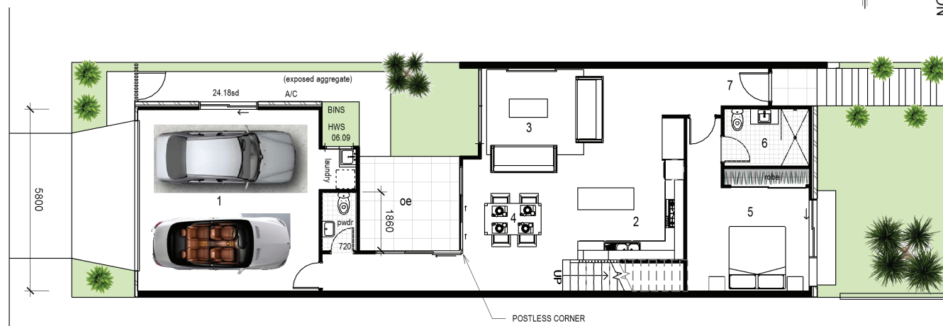
LOWER FLOOR PLAN
